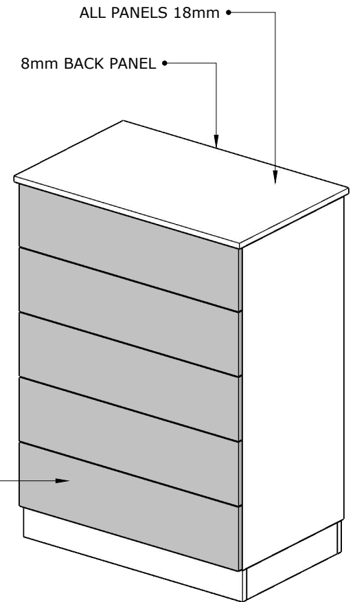
FIVE DRAWER DOUBLE CHEST
